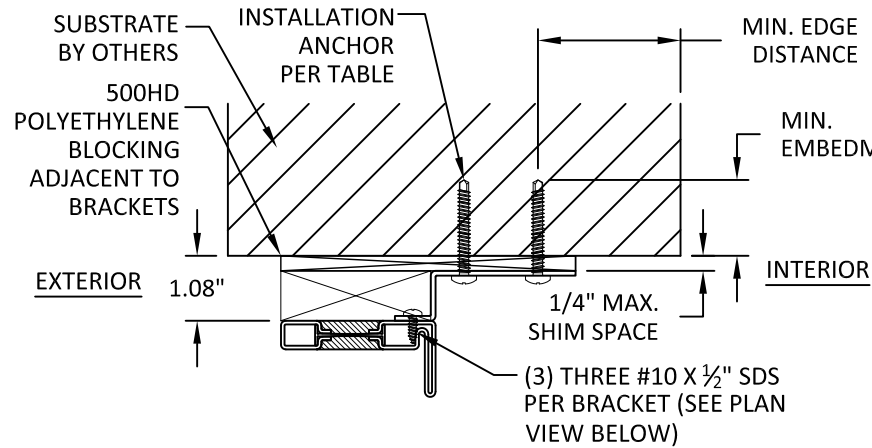
B 4 ANCHOR DETAIL BRACKET
