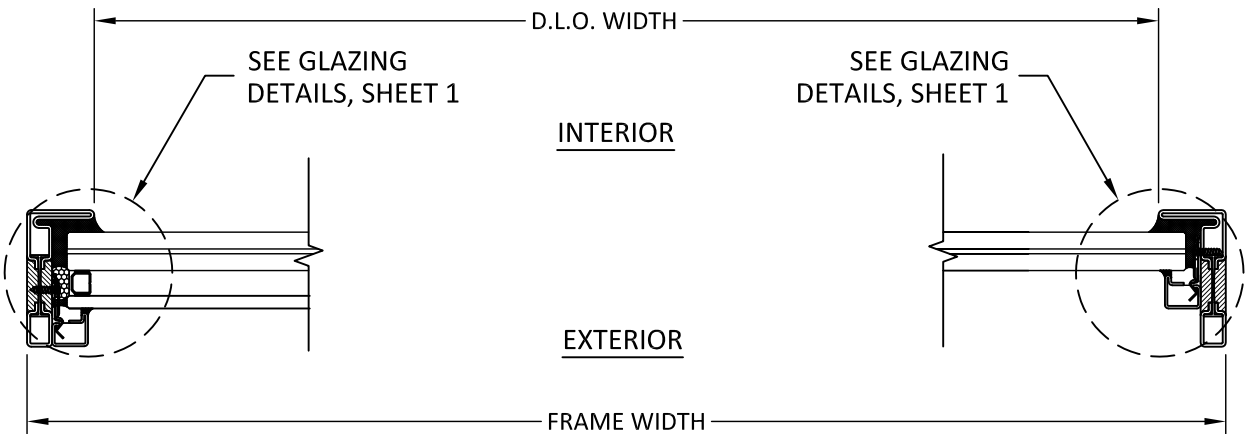
HORIZONTAL SECTION JAMB - OUTSIDE GLAZED
