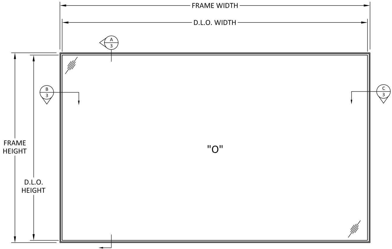
ELEVATION RECTANGULAR O
