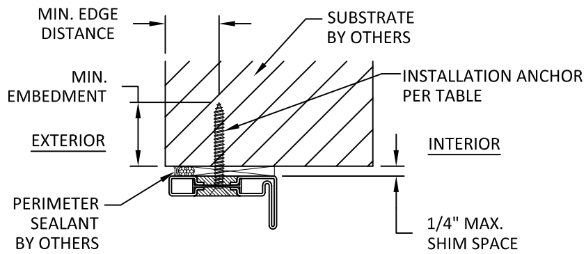
A 4 ANCHOR DETAIL THROUGH FRAME
